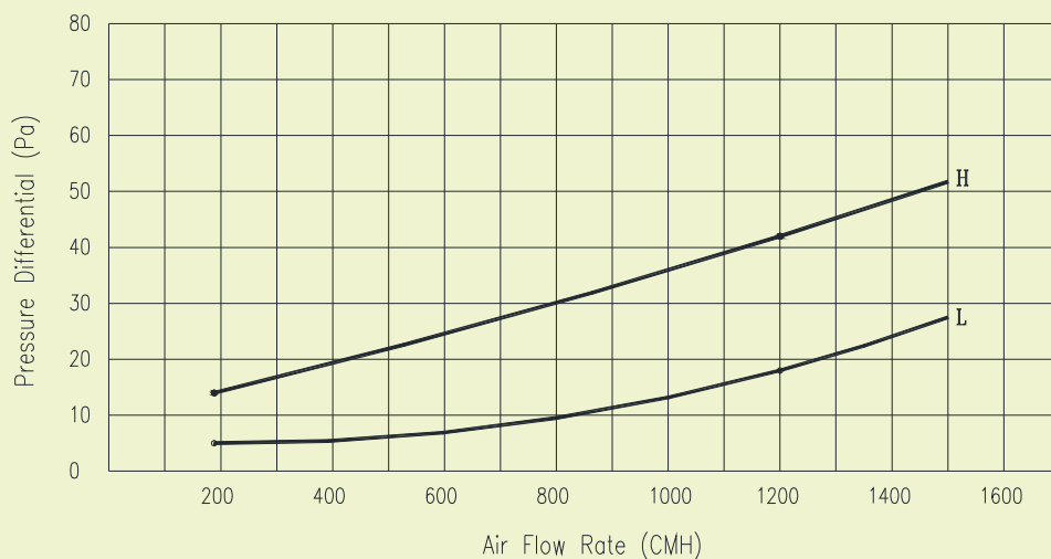
PERFORMANCE CURVE: VPRD-20
