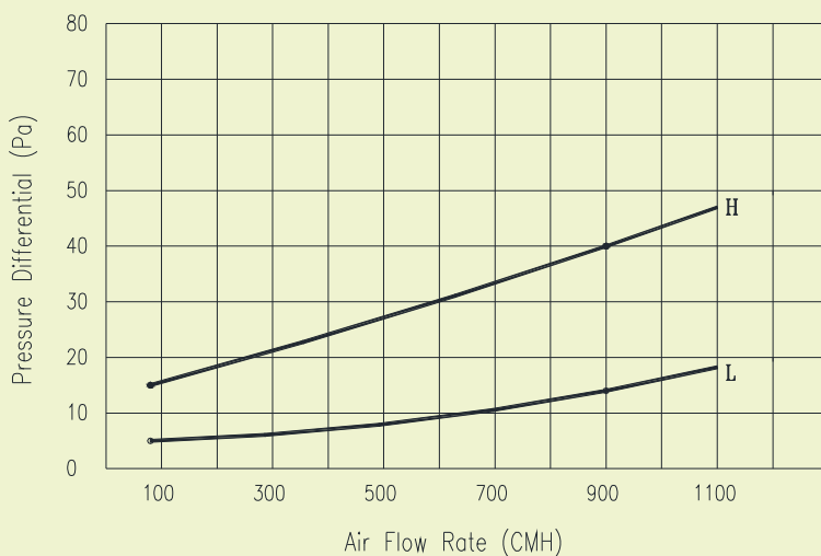
PERFORMANCE CURVE: VPRD-15
